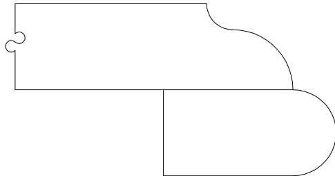
Ogee & Full Bullnose
